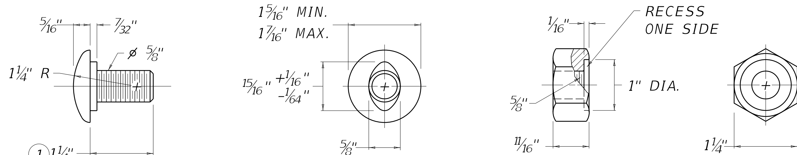
5/8" BUTTON HEAD BOLT AND RECESSED NUT
