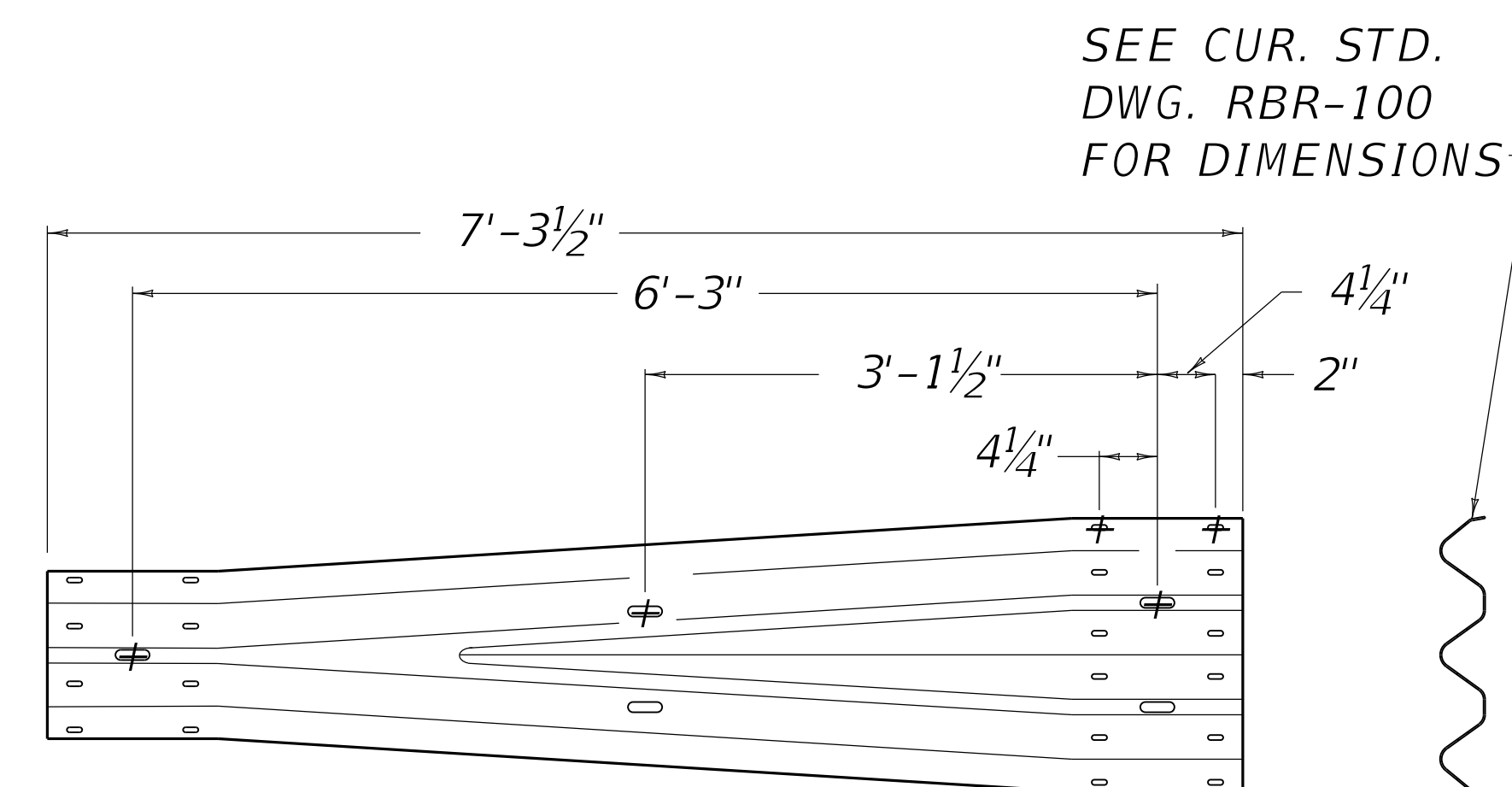
THRIE BEAM TO "W" BEAM CONNECTOR (2)
